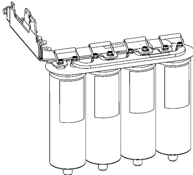
Figure 1 – New Bus Bar and Capacitor Bank Assembly (TT300/TG230 Only)
