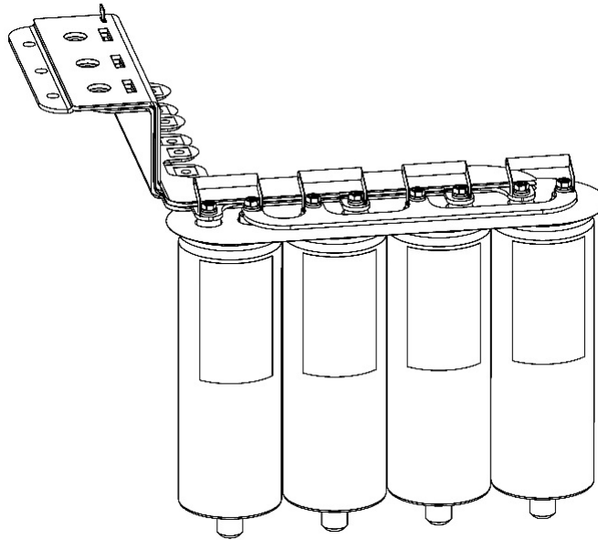
Figure 2 – New Bus Bar and Capacitor Bank Assembly (All TT/TG Compressors Except TT300/TG230)
