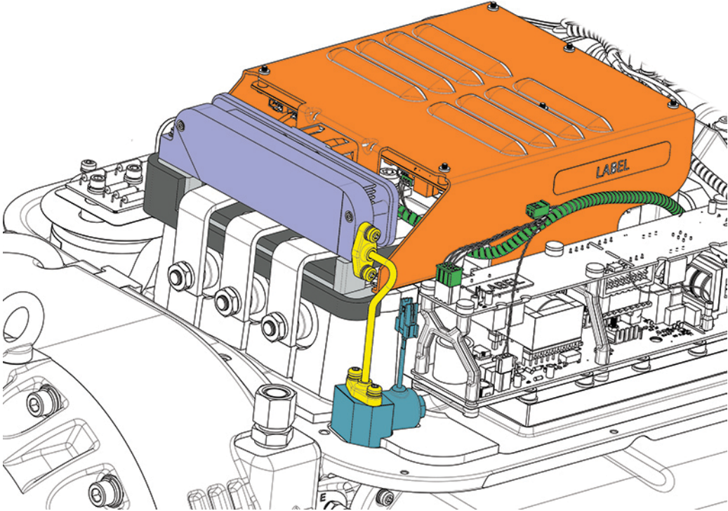
Figure 4-2 Active Cooling Components
